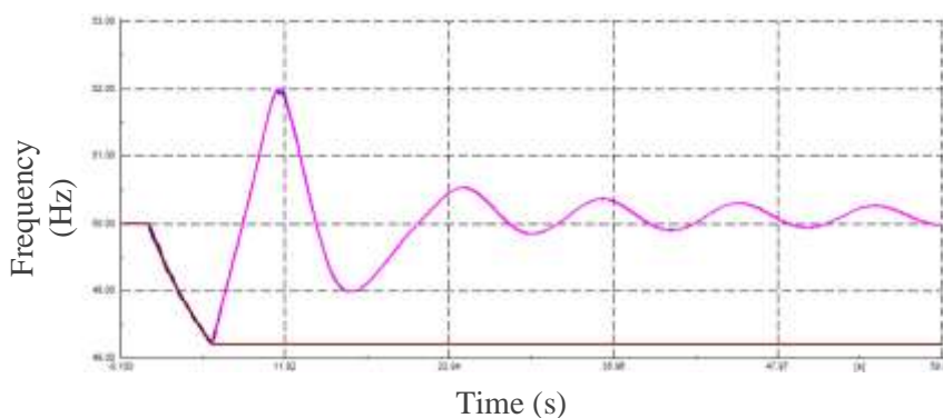
Figure 8. System’s frequency performance if both Sidrap and Jenepono WPPs are out of the system at 150 kV buses.
