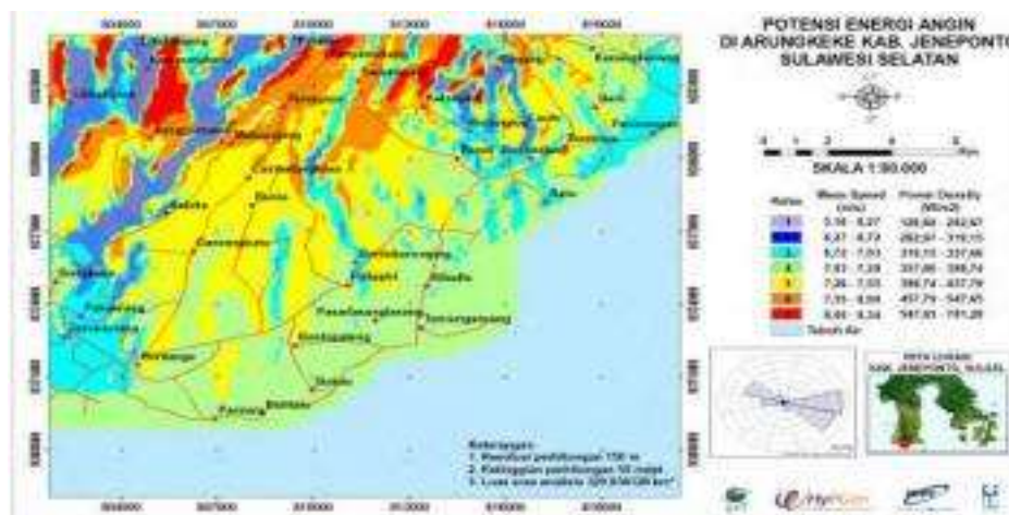
Figure 2. Wind energy potential at Jeneponto Regency [9]
