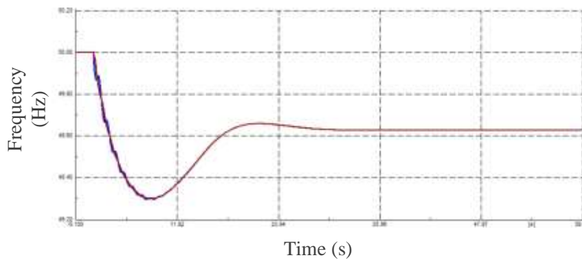
Figure 6. System’s frequency performance if Jenepono WPPs are out of the system at 150 kV buses
