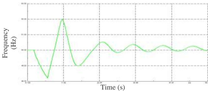
Figure 7. System’s frequency performance if both Sidrap and Jenepono WPPs are out of the system at 275 kV buses.
