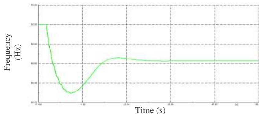
Figure 5. System’s frequency performance if Jeneponto WPPs are out of the system at 275 kV buses
